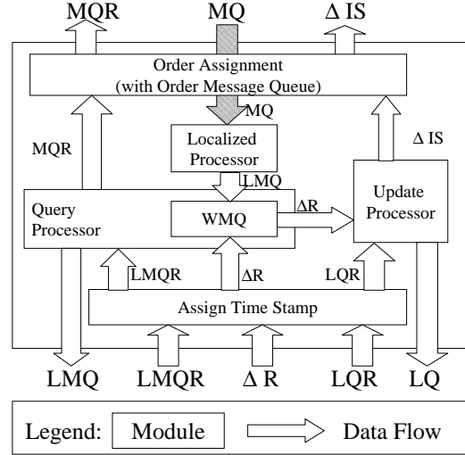
Figure 4: Architecture of the MRE Wrapper
